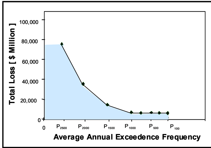
Figure C-1. Probabilistic Loss Curve
