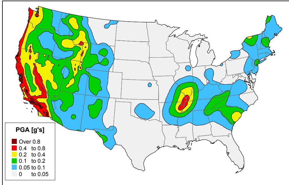
Figure 2-2. USGS Seismic Hazard Map for 1000-year Return Period
