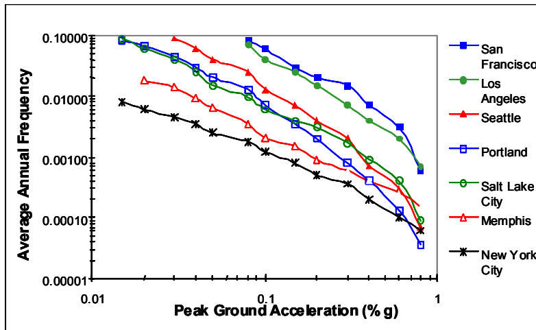
Figure 2-1. Average Annual Frequency of Peak Ground Acceleration for Seven Major Cities
