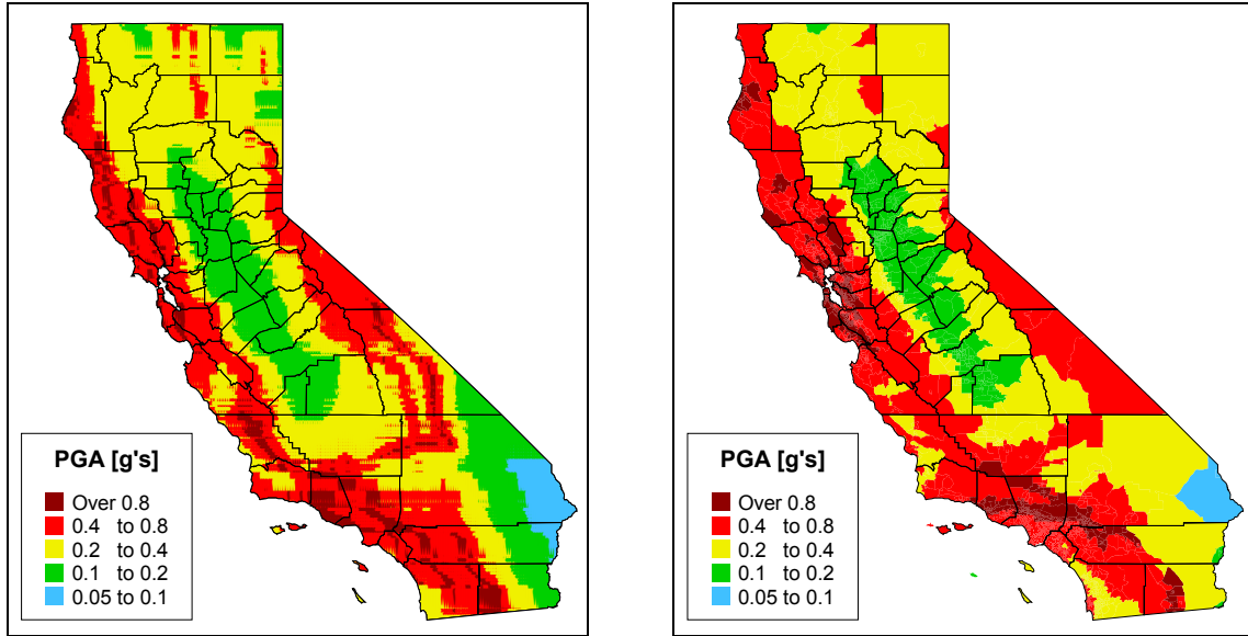
Figure 2-3. Comparison of HAZUS Seismic Hazard Map for PGA in g's (left) and USGS Hazard Map (right) for 1000-year Return Period Ground Motion in California for a B/C soil
